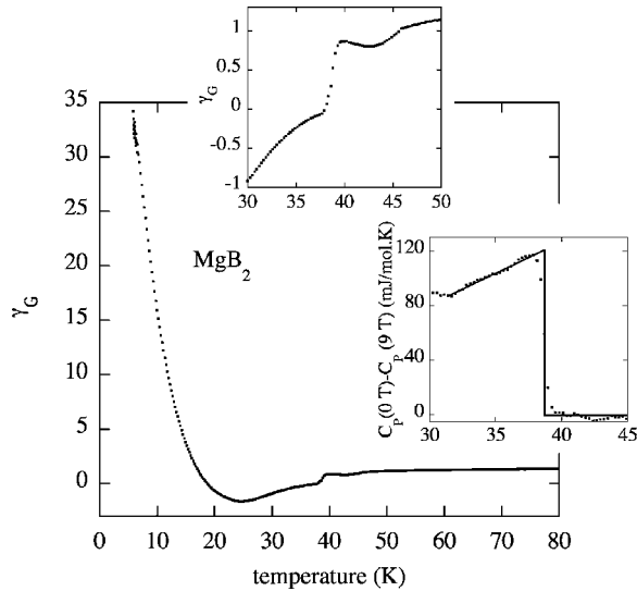
FIG. 4. The main panel and upper inset show the bulk Grüneisen function \gamma_G versus temperature. The lower inset shows heat capacity C_p after subtraction of C_p(9 \text{ tesla}) ; the solid line indicates the jump expected for a continuous (second-order) phase transition.
